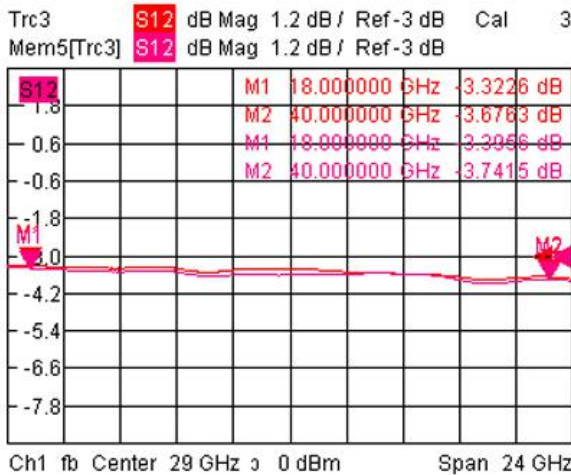
3.插入损耗 Insertion Loss
